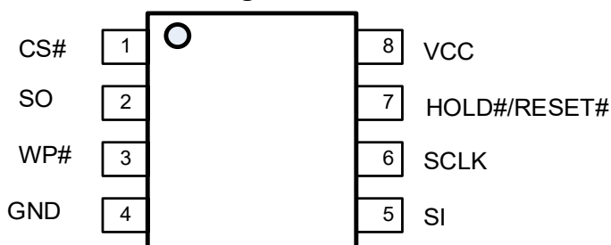
8-Lead SOP (150mil) and TSSOP
