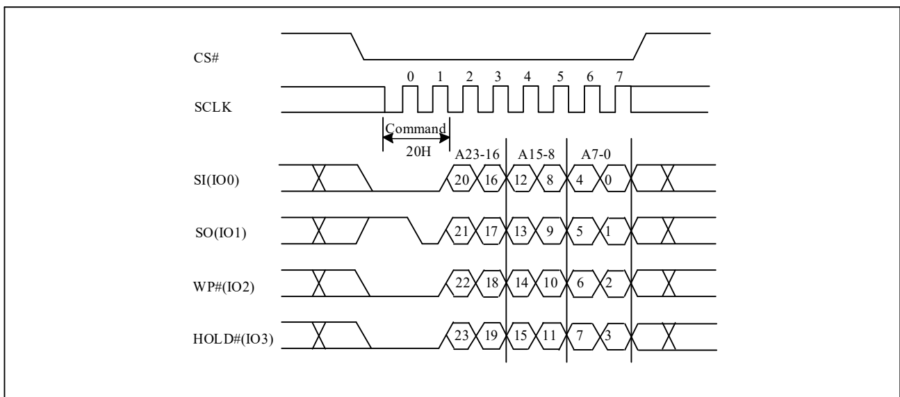
Figure 10-22a Sector Erase (SE) Sequence (QPI)
