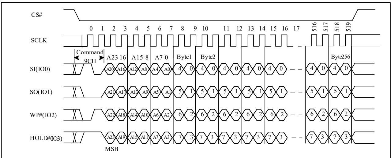
Figure 10-31a Buffer Write Sequence (QPI)
