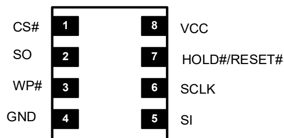
8-Pad USON (1.5x1.5mm/3x2mm)
