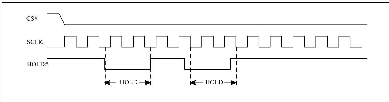
Figure 89 Hold Condition Operation
