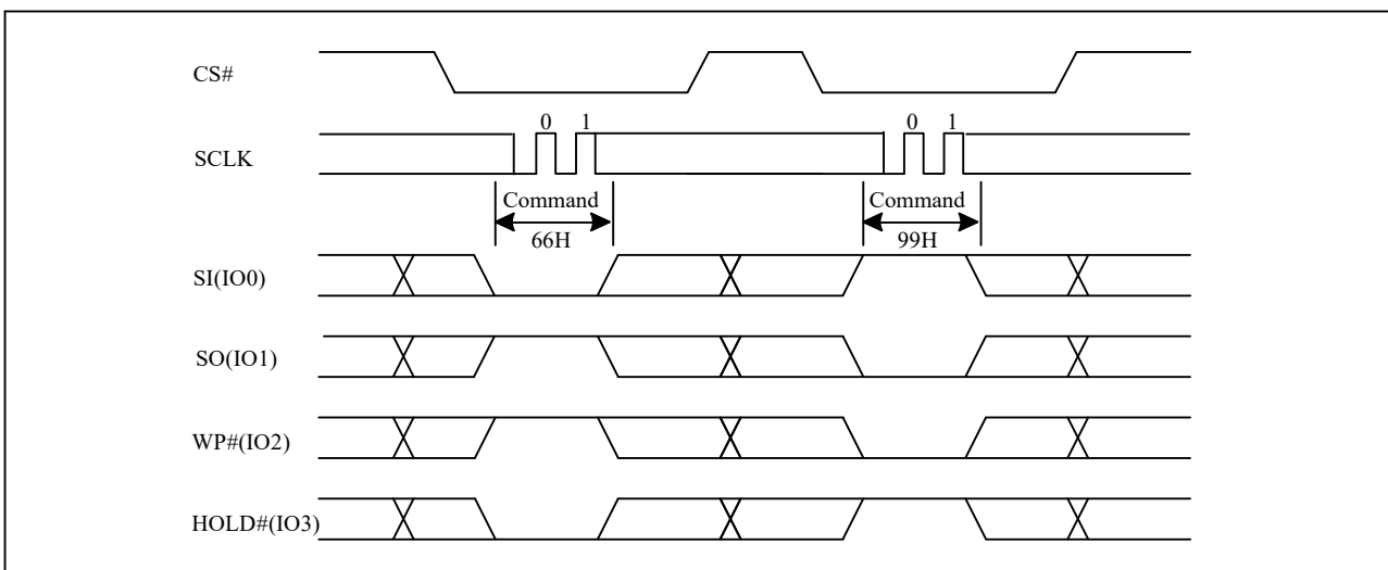
Figure 10-51c Reset Sequence(QPI)
