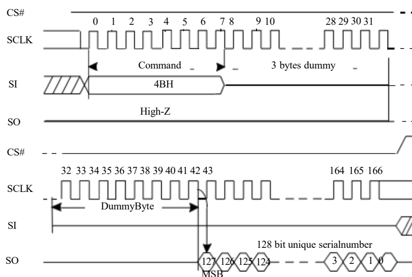
Figure 29. Read Unique ID Sequence Diagram
