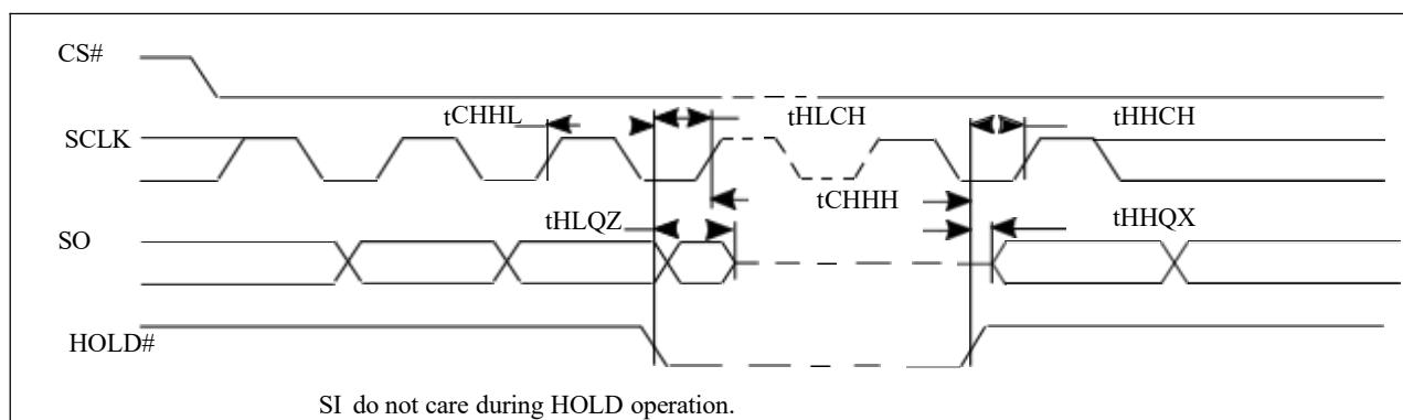
Figure43. Hold Timing
