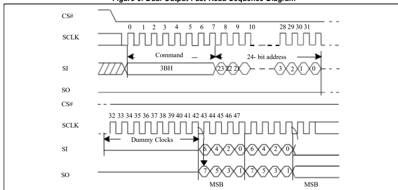
Figure 9. Dual Output Fast Read Sequence Diagram
