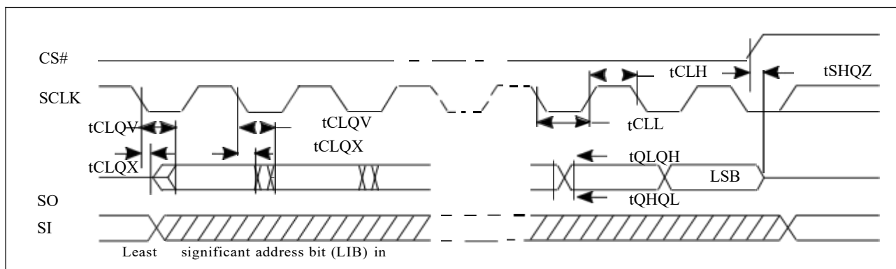
Figure 42. Resume to Suspend Timing Diagram
