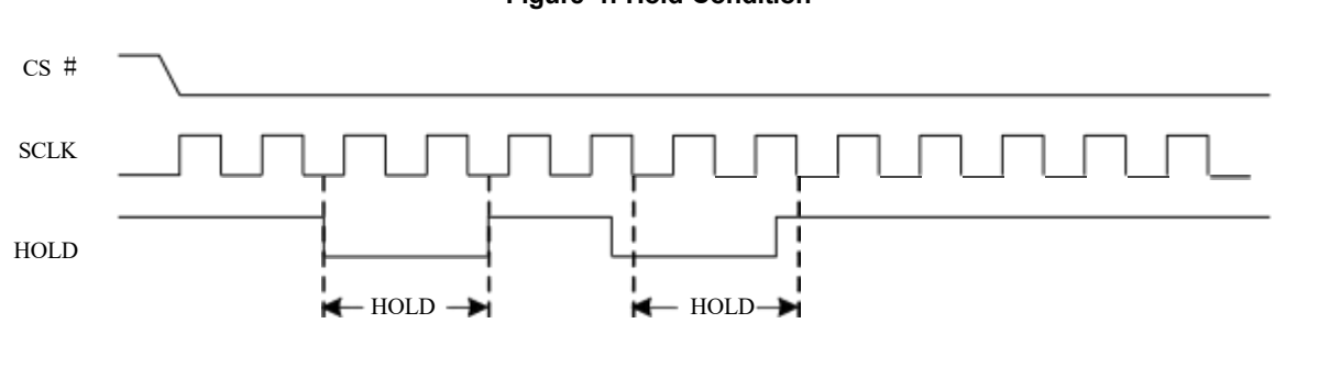
Figure 1. Hold Condition
